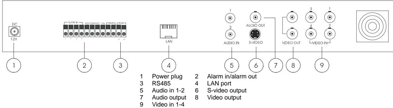
Fig2.2 Back Panel
