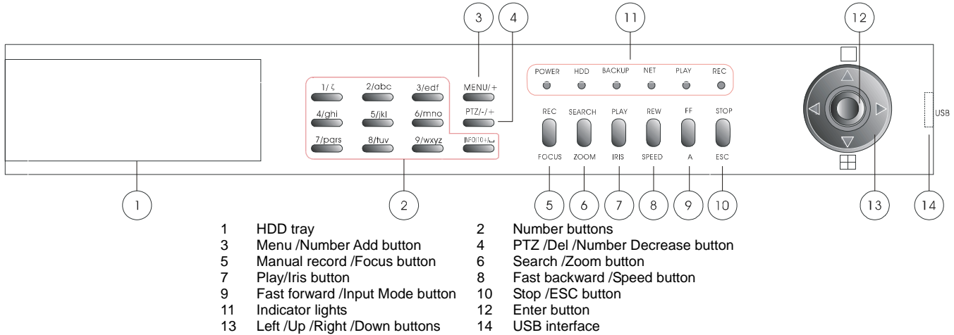
Fig2.1 Front Panel
